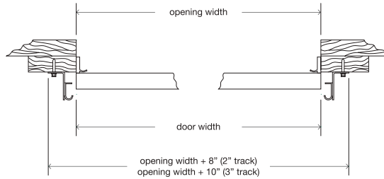
BRACKET MOUNTED TRACK: LEG OUT (WOOD JAMBS SHOWN)
