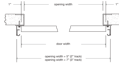
REVERSE ANGLE TRACK: LEG IN (STEEL JAMBS SHOWN)
