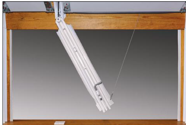
Swing-Up Post
